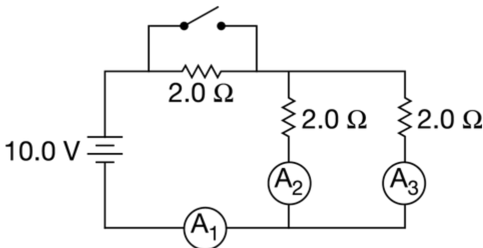
Figure 1. When the switch is open
