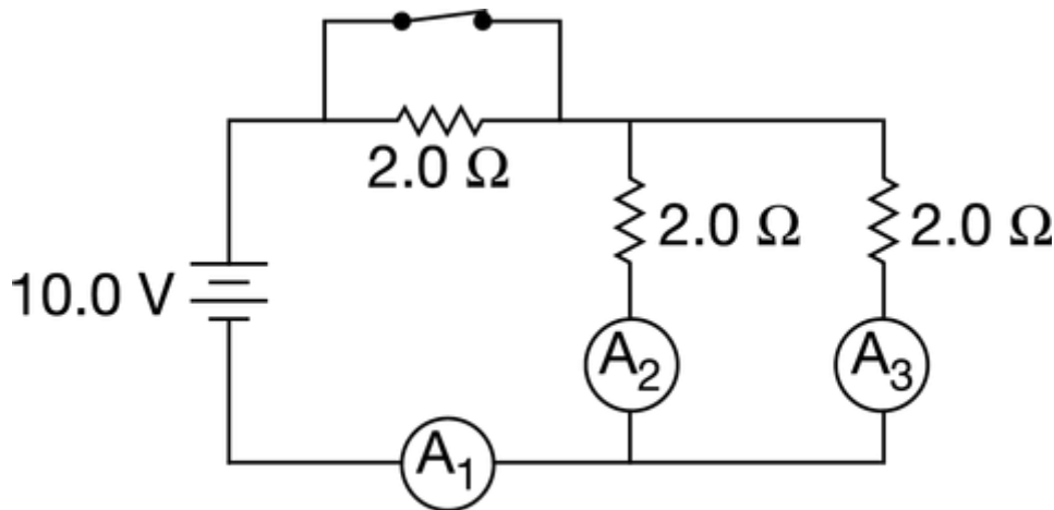
Figure 2. When the switch is closed
